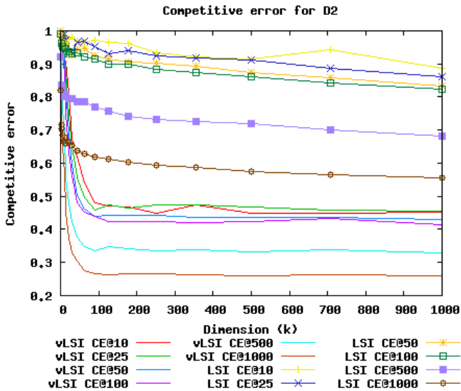
Figure 5: LSI and VLSI over 1000 dimensions with query distribution D1 (above) and D2 (below) measured by competitive error at 10 through 1000 documents. Plots with points correspond to LSI; those without points correspond to VLSI.
